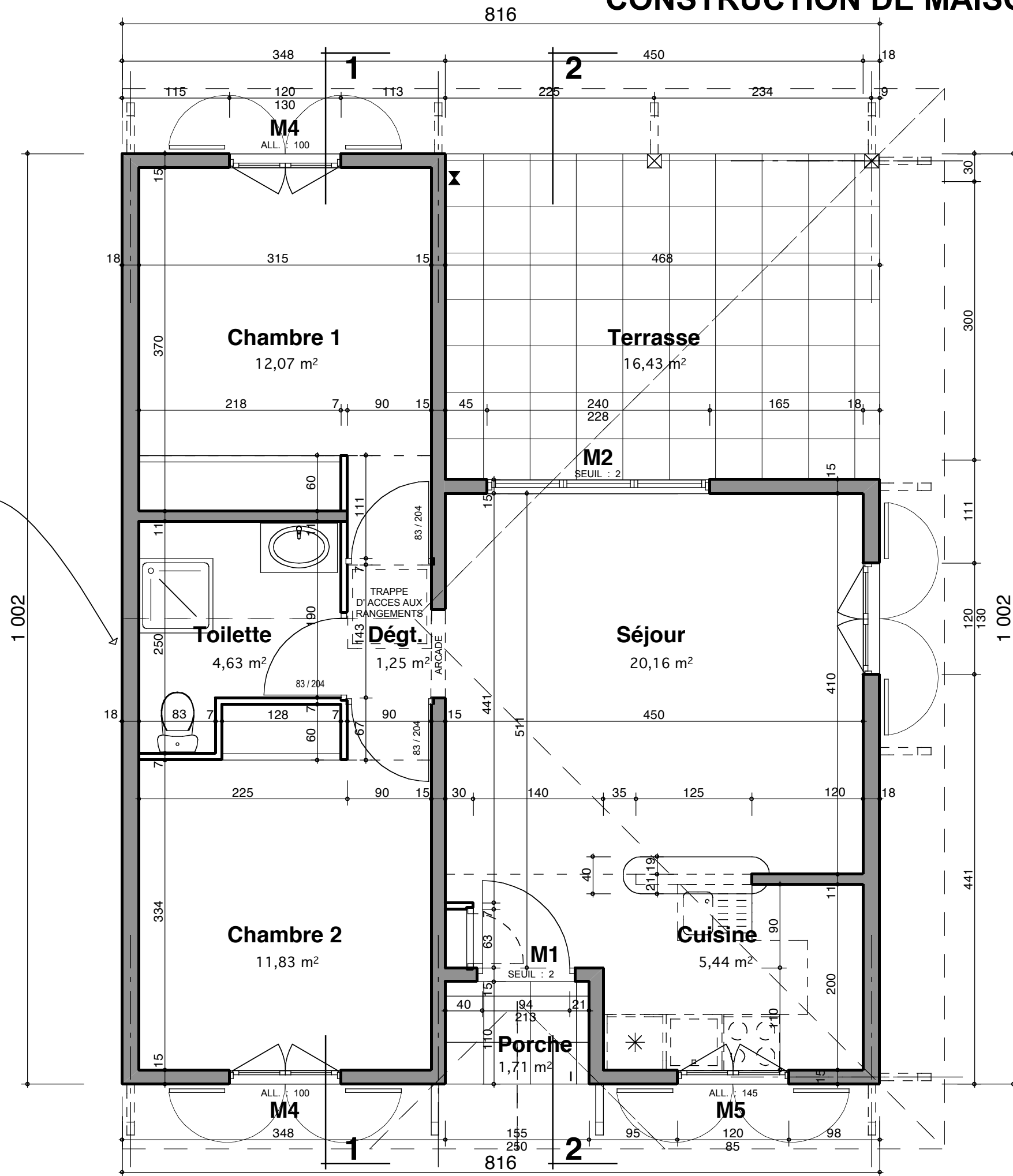
Type F3 - 73,52m 2
